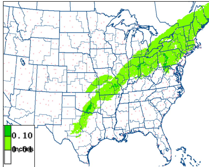
Ice Accumulation through Friday Morning
