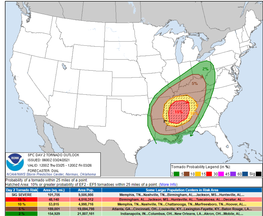
Tornado Outlook
