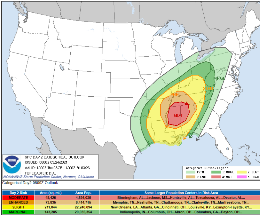
Categorical Outlook
