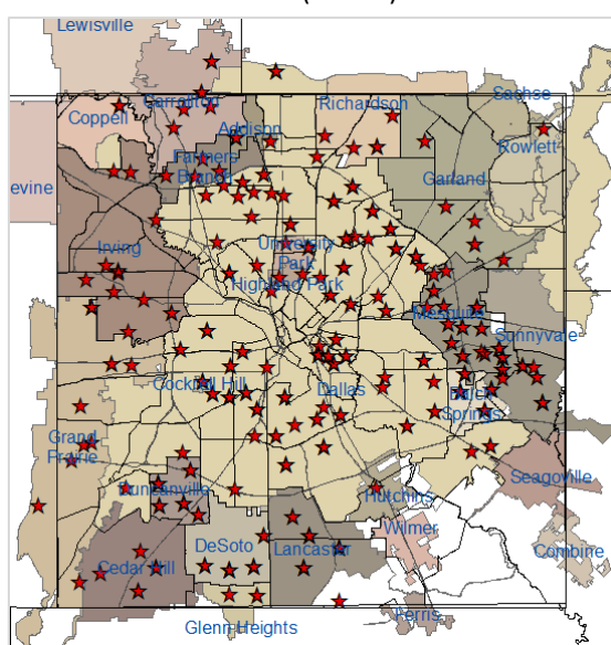
Figure 2: Cumulative WNV Positive Mosquito Traps Collected: Weeks 1-35* (N=339)
