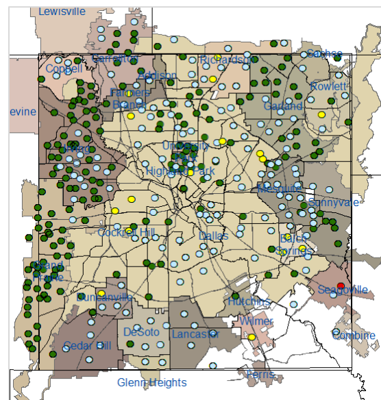
Figure 4: Trap Counts of Female Cx. quinquefasciatus from 2020 Season: Weeks 1-35*
