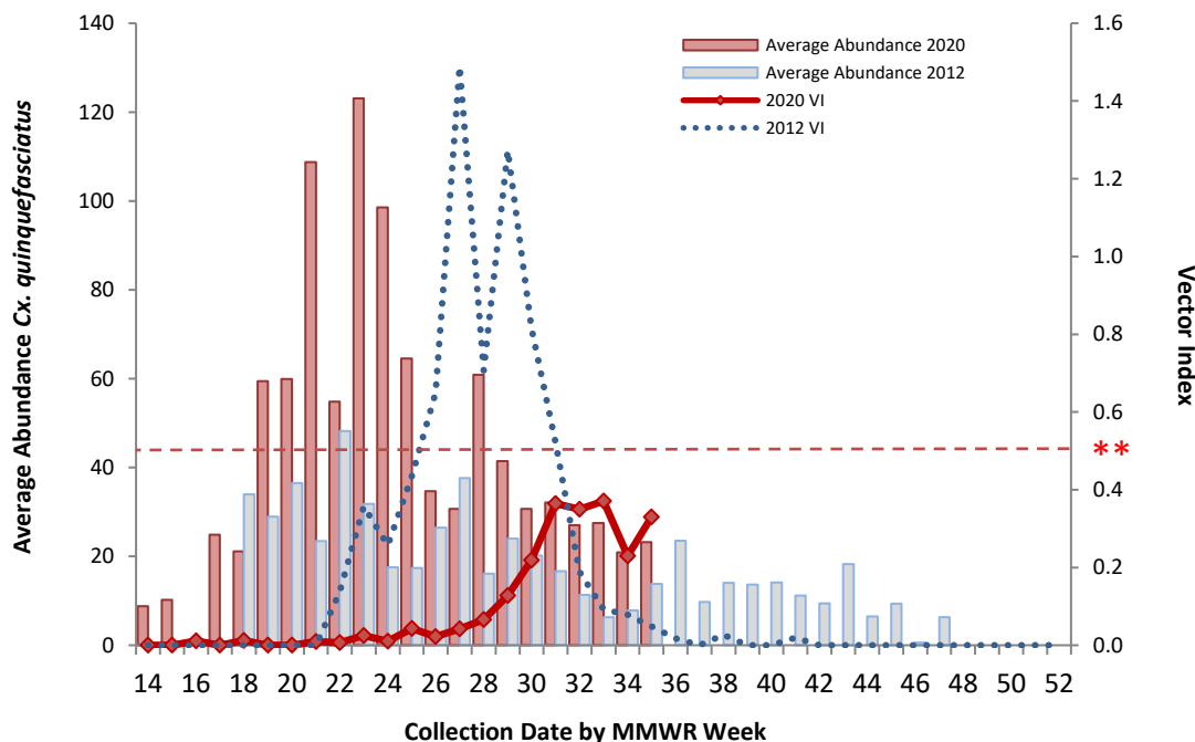
Figure 5: Average Numbers of Female Cx. quinquefasciatus per Trap-night and WNV Vector Index by Week: 2012 Season and 2020 Season (through Week 35*)
