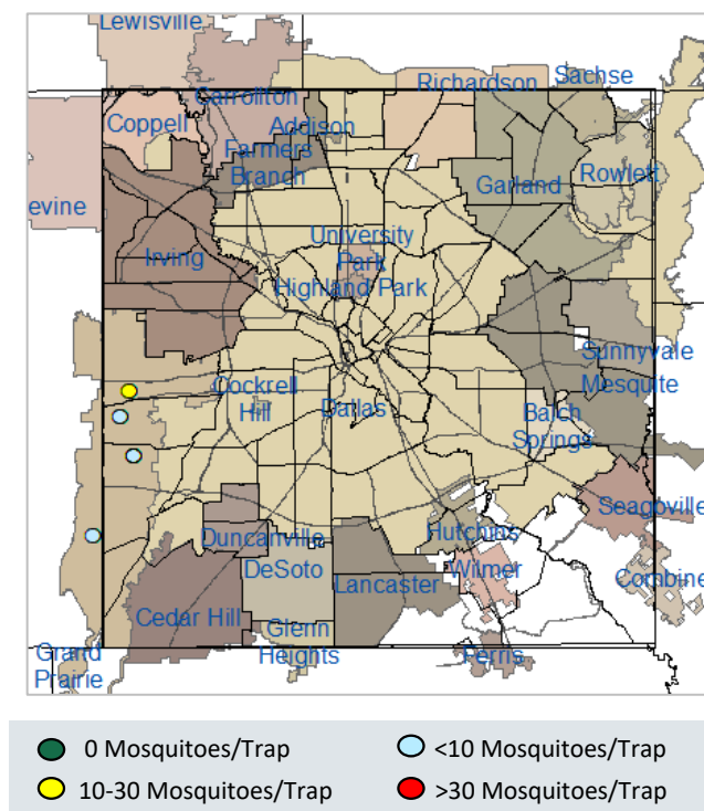
Figure 9: BG-Sentinel Trap Counts of Female Aedes aegypti and Aedes albopictus during 2020: Weeks 15 through 35 †
