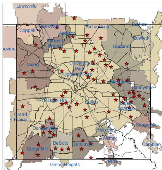
Figure 3: WNV Positive Mosquito Traps Collected During 2020: Weeks 34 and 35* (N=89)
