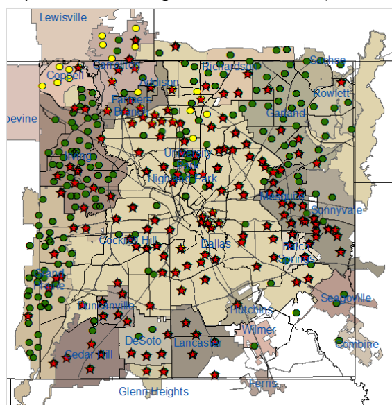
Figure 1: All WNV Negative and Positive Mosquito Traps Collected During 2020: Weeks 1-35* (N=5,174)
